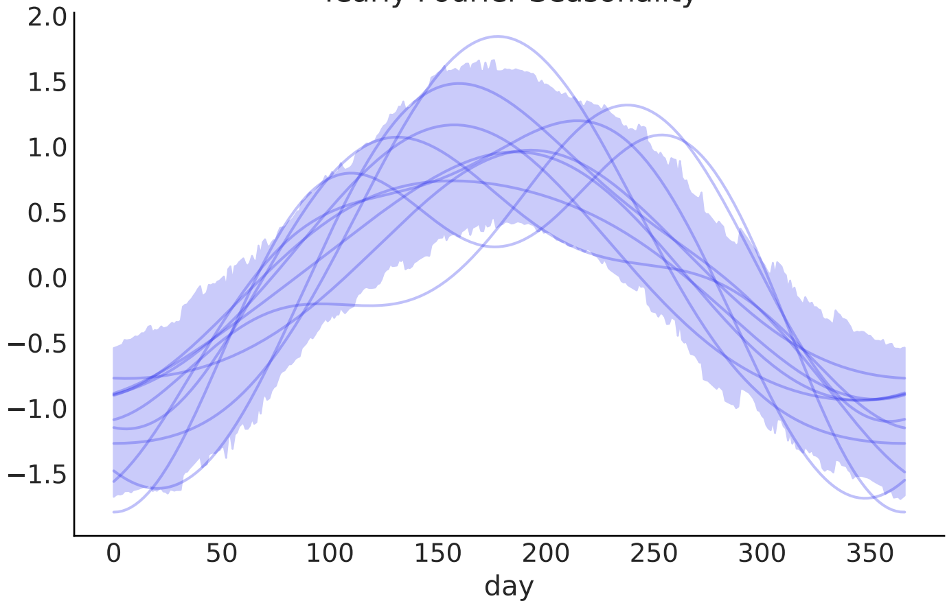
Yearly Fourier Seasonality
